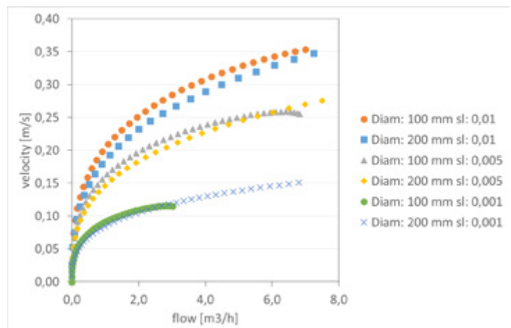
Figure 1 Relation between velocity, flow, diameter and slope for partially filled pipes. The flow is relevant for maximum domestic water use (and waste water production) for 20-40 houses.
