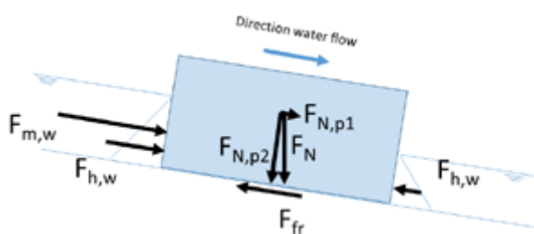
Figure 2 Forces on an object in a sloped pipe
